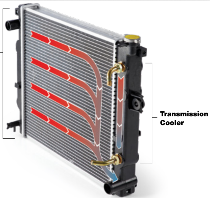
Engine Radiator
