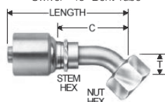
Female Flat-Face Swivel - 45° Bent Tube
