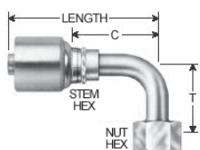
Female Flat-Face Swivel - 90° Bent Tube, O-Ring Face Seal
