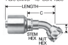
Female JIC 37° Flare Swivel - 45° Bent Tube
