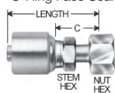
Female Flat-Face Swivel, O-Ring Face Seal
